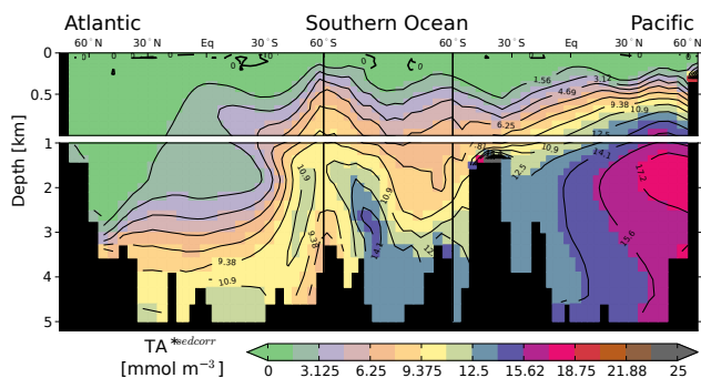
Figure 3. Influence of ocean–sediment fluxes on TA*. The mean offset in TA* between simulations with and without the sediment module is shown for the 14 ensemble members with the highest skill. Displayed are results for a cross section through the Atlantic (25° W), across the Southern Ocean (58° S) into the Pacific, and through the Pacific (175° W). Note the colour bar.
