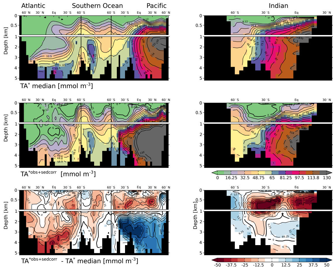
Figure 5. Observation-based vs. simulated TA*. Left column: modelled (median) TA*, observed TA*, and their difference in a cross section through the Atlantic (25° W), Southern Ocean (58° S), and Pacific (175° W). Right column: the same for a cross section along 95° E in the Indian Ocean. The correlation coefficient, relative standard deviation ( \sigma_{rel}^{obs} ), and root mean square error (RMSE) between the simulated and observation-based fields are 0.83, 1.09, and 17.7 mmol m -3 in the Atlantic; 0.88, 0.8, and 23.8 mmol m -3 in the Pacific; 0.87, 0.86, and 19.8 mmol m -3 in the Indian Ocean.
