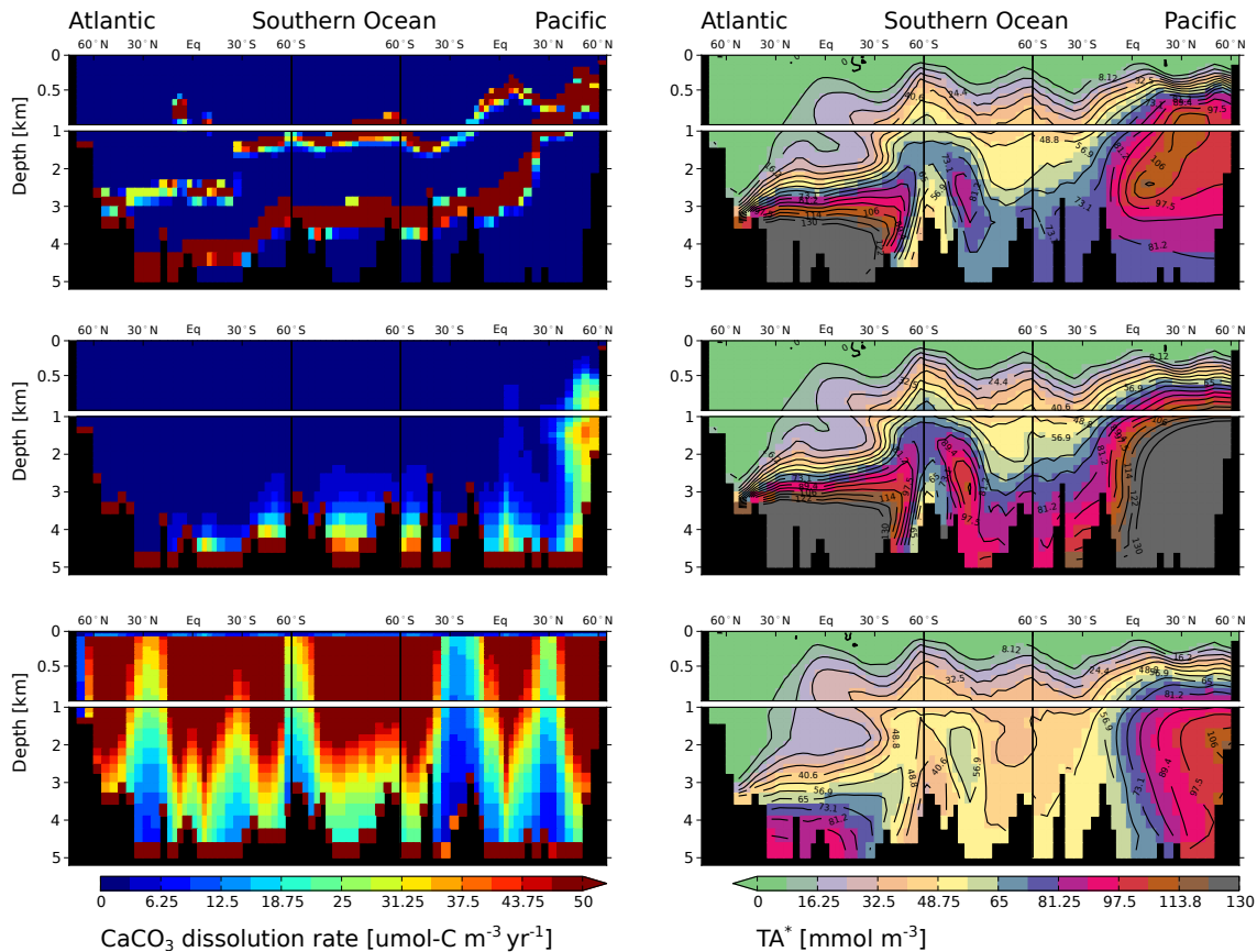
Figure 2. Results from sensitivity simulations applying three different illustrative dissolution schemes. Left column: \text{CaCO}_3 dissolution rates. Right column: the resulting steady-state \text{TA}^* for these three contrasting parameterisations of the \text{CaCO}_3 dissolution rate. The dissolution rate is set to increase fast (top row), slowly (middle row) with undersaturation of \text{CaCO}_3 , or is set constant throughout the water column (bottom row). The standard version of the Bern3D model without the sediment module is applied, and the fraction of \text{CaCO}_3 export in the form of aragonite is set to 10 %. At least 43 % of the dissolution signal is simulated above the calcite saturation horizon irrespective of whether dissolution is allowed to occur above the saturation horizon (bottom row) or not (middle and top row). This points to the importance of physical transport in shaping the distribution of \text{TA}^* .
