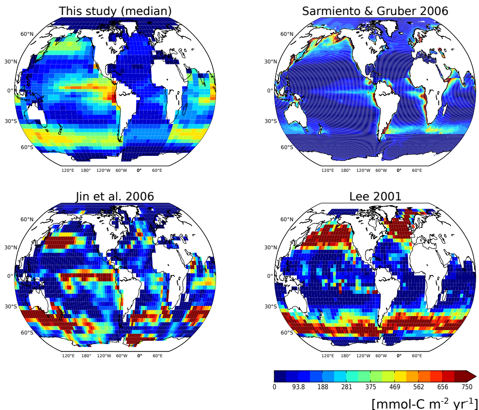
Figure 10. Observationally constrained CaCO 3 export fields as estimated by different studies. Global total export is estimated to be 0.5 by Sarmiento and Gruber (2006), 1.14 by Jin et al. (2006), 1.1 by Lee (2001), and 0.90 Gt C yr -1 by this study.
