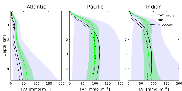
Figure 4. Model ensemble vs. observation-based basin-mean TA* profiles. The grey shading shows the unconstrained prior and the green shading shows the constrained (68 % confidence interval) distribution of the model ensemble. Lines represent the median of the constrained ensemble (green), observation-based TA* (black dashes), and observation-based TA* corrected for a sediment burial flux of 0.12 Gt C yr -1 (black solid). The corresponding Southern Ocean sector is included in the averaging.
