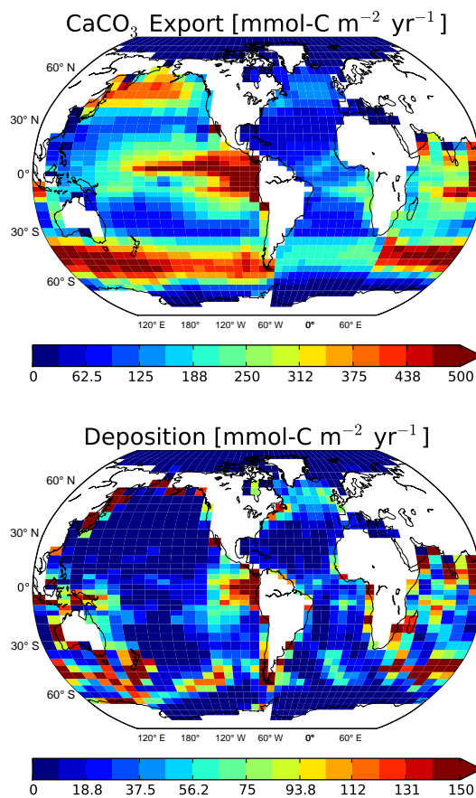
Figure 7. Top: median \text{CaCO}_3 export, globally 0.90 (0.72\text{--}1.05) \text{ Gt C yr}^{-1} . Bottom: median \text{CaCO}_3 fluxes reaching the ocean floor, globally 0.164 (0.113\text{--}0.227) \text{ Gt C yr}^{-1} . Note the different scaling of the colour bars.
