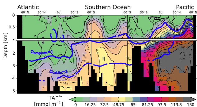
Figure 1. The TA* tracer captures exclusively the influence of CaCO 3 dissolution on alkalinity. An observationally based estimate of the TA* distribution (mmol m -3 ) yielding an inventory of ~ 37.5 Pmol C of which ~ 41 % comes to lie above the calcite saturation horizon. The calcite ( \sigma_{\text{calcite}}=1 ) and aragonite ( \sigma_{\text{aragonite}}=1 ) saturation horizon are shown by the blue lines. Displayed are results for a cross section through the Atlantic (25° W), across the Southern Ocean (58° S) into the Pacific, and through the Pacific (175° W).
